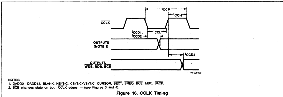
Figure 16. CCLK Timing
