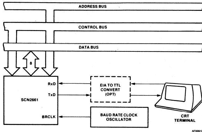
Asynchronous Interface to CRT Terminal
