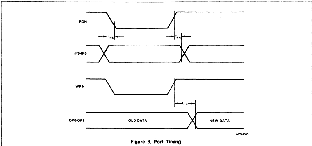
Figure 3. Port Timing
