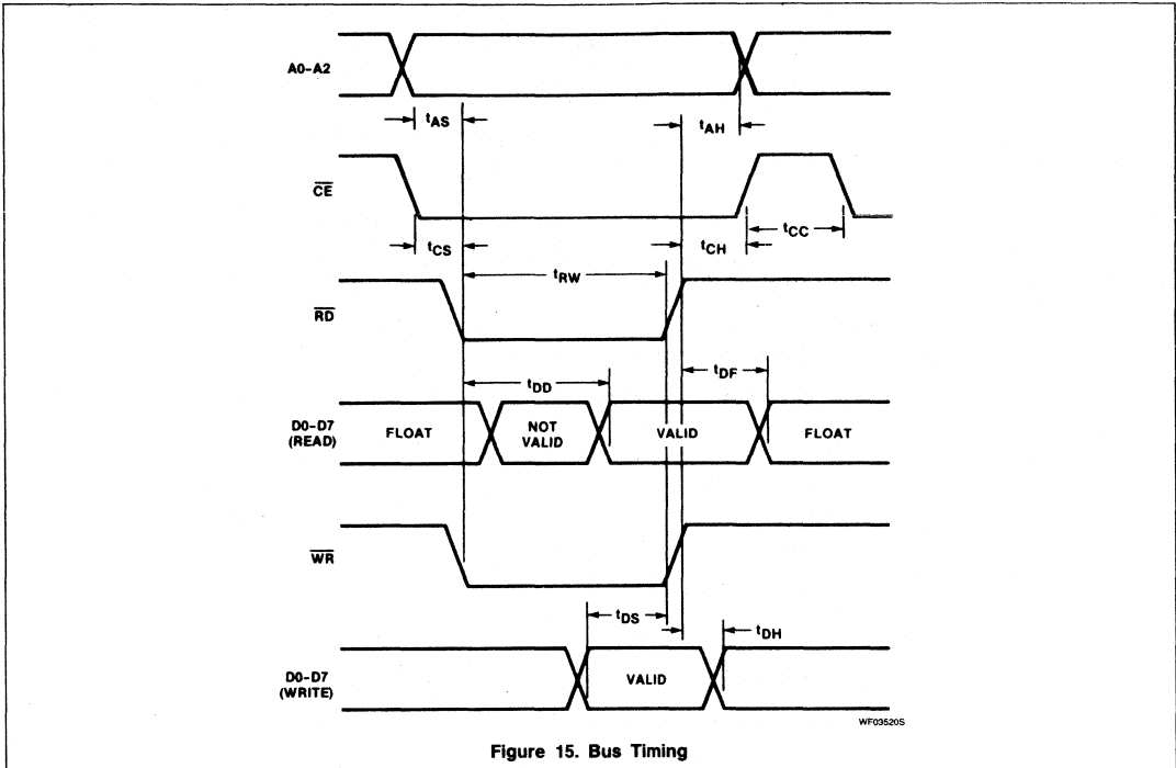
Figure 15. Bus Timing
