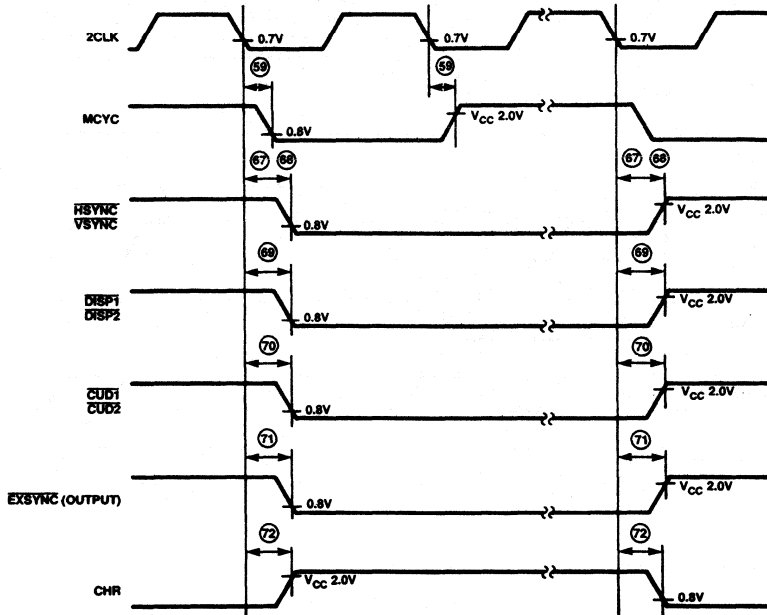
Figure 50. Display Control Signal Output Timing
