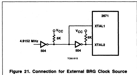
Figure 21. Connection for External BRG Clock Source
