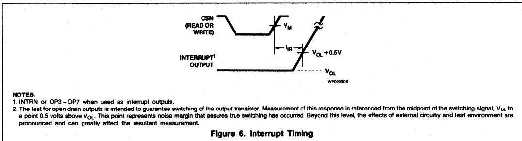
Figure 6. Interrupt Timing
