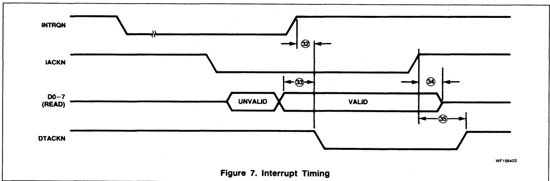
Figure 7. Interrupt Timing
