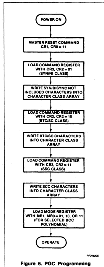
Figure 6. PGC Programming
