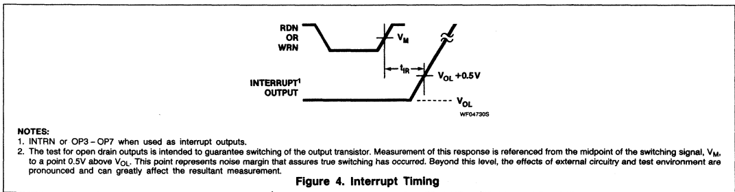
Figure 4. Interrupt Timing
