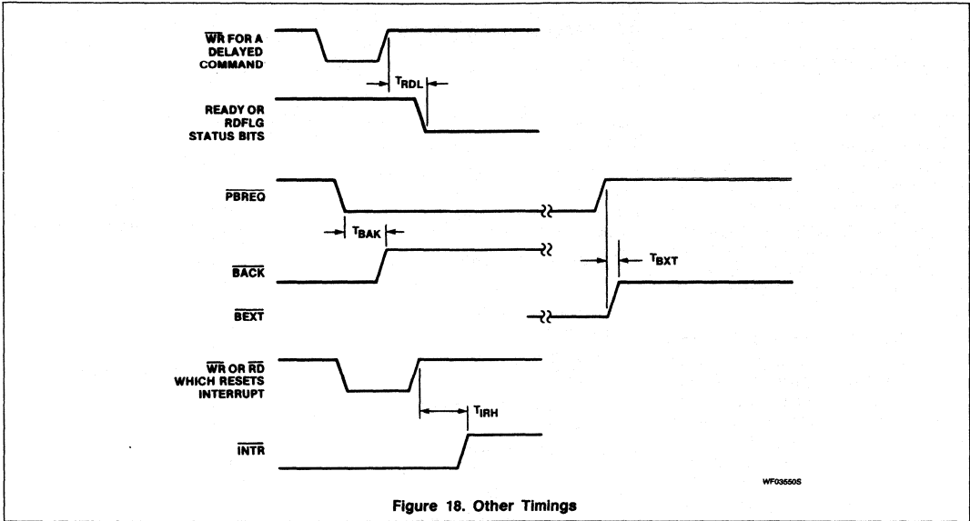
Figure 18. Other Timings
