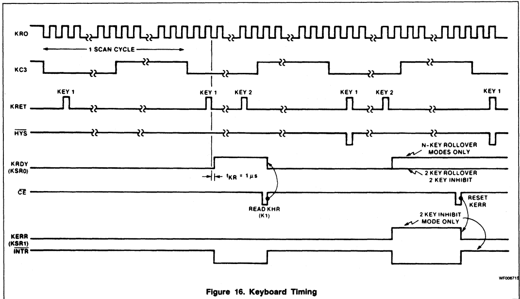
Figure 16. Keyboard Timing
