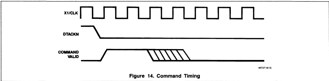
Figure 14. Command Timing
