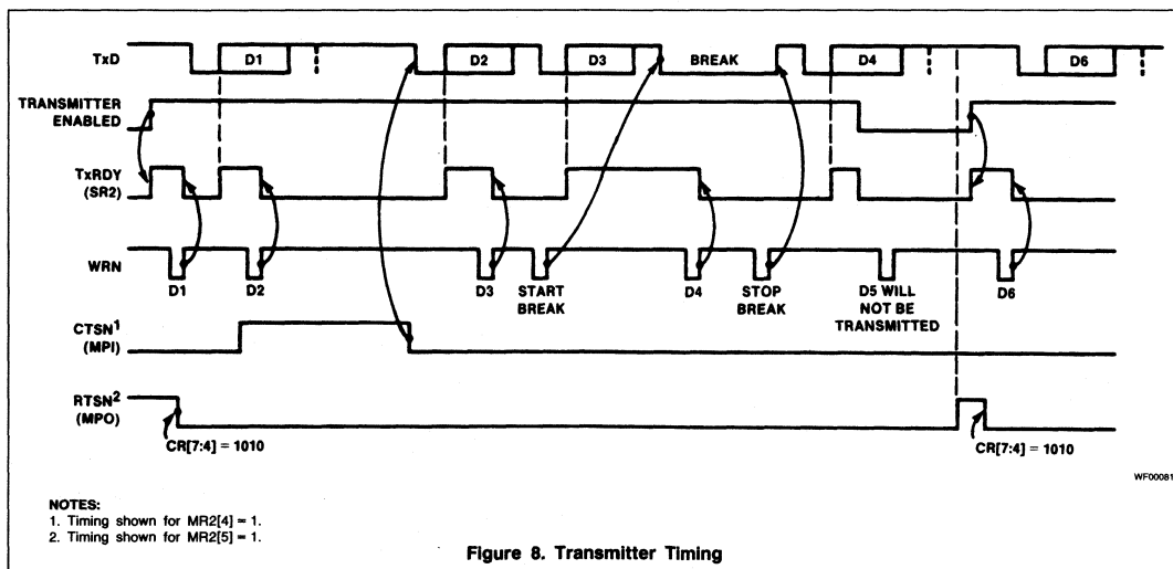
Figure 8. Transmitter Timing
