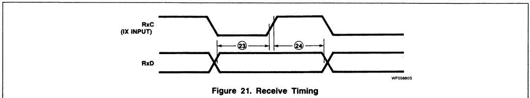
Figure 21. Receive Timing
