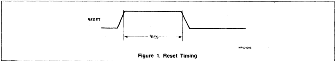
Figure 1. Reset Timing
