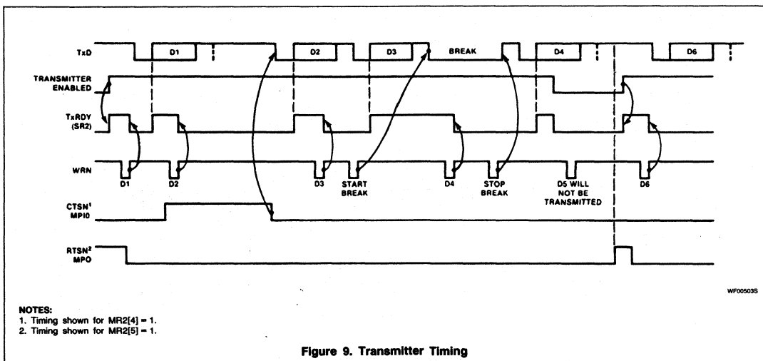
Figure 9. Transmitter Timing
