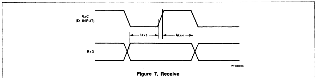
Figure 7. Receive
