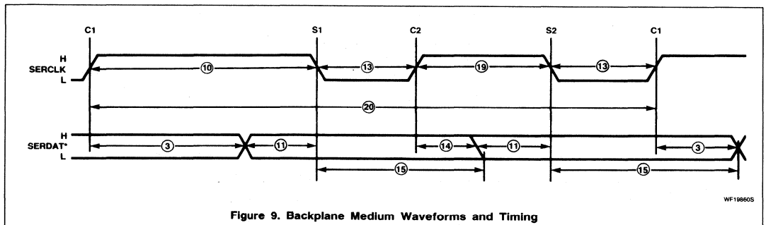
Figure 9. Backplane Medium Waveforms and Timing
