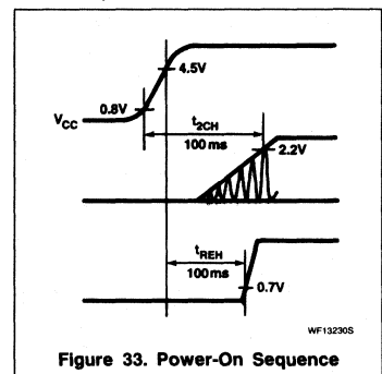
Figure 33. Power-On Sequence
