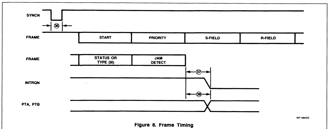
Figure 8. Frame Timing
