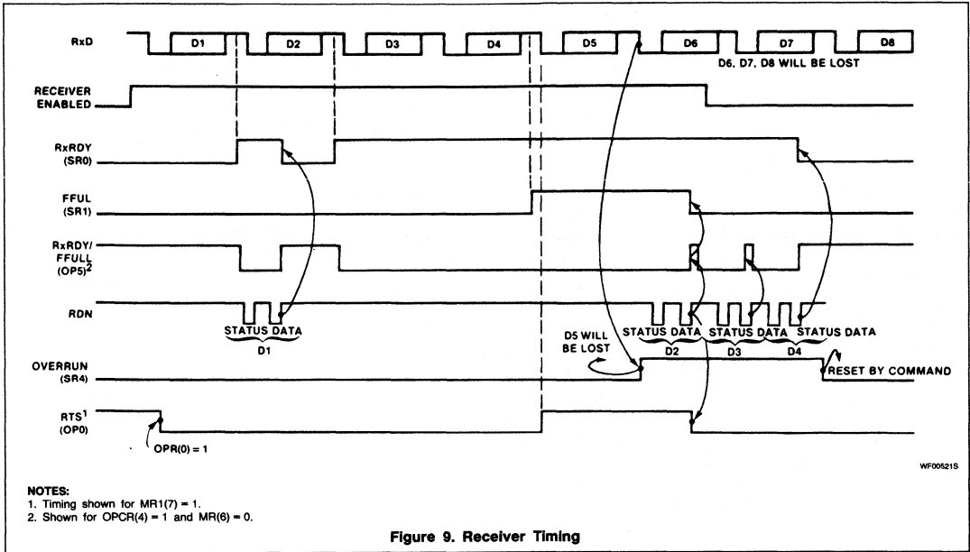
Figure 9. Receiver Timing
