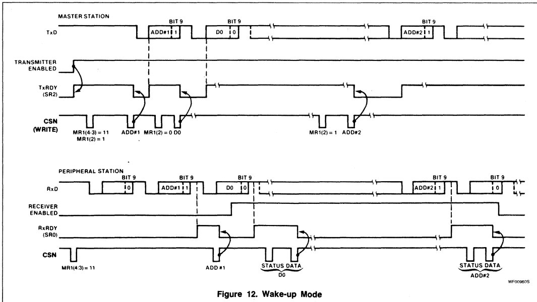
Figure 12. Wake-up Mode
