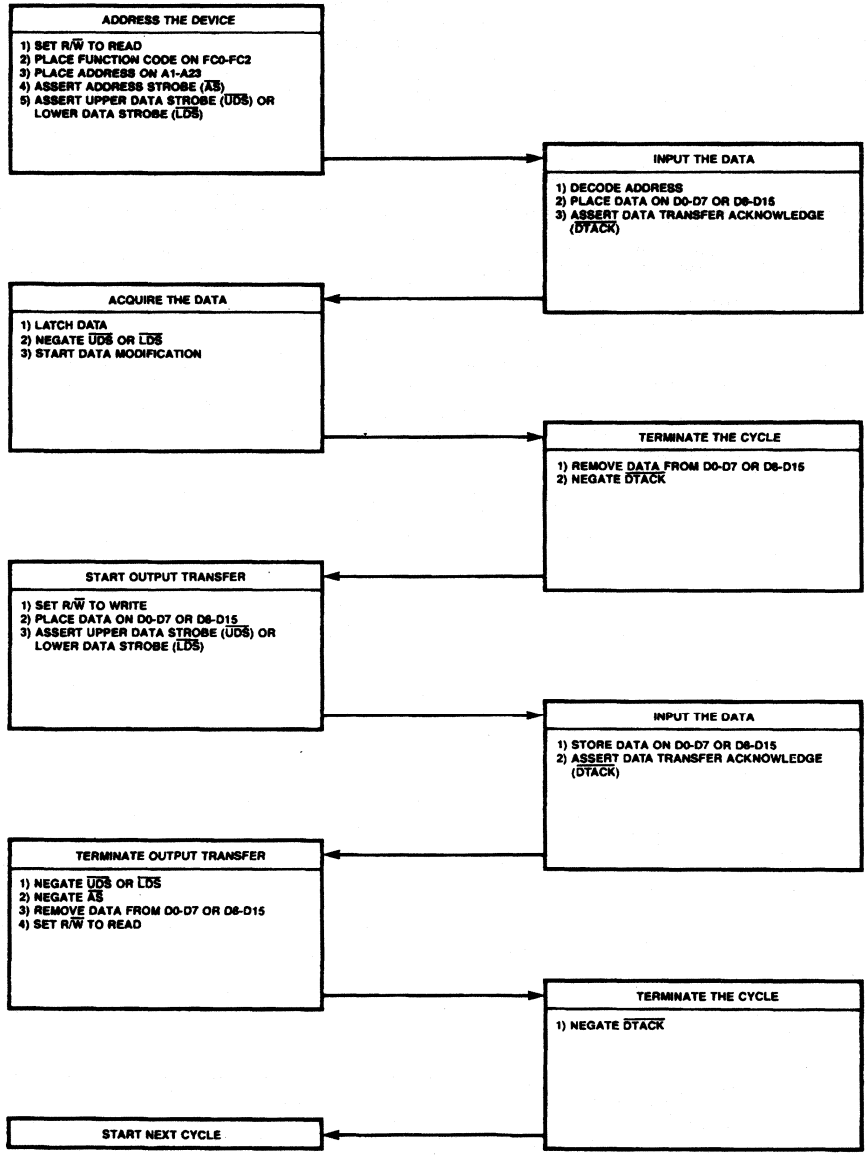
Figure 16. Read-Modify-Write Cycle Flowchart
