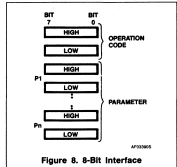
Figure 8. 8-Bit Interface
