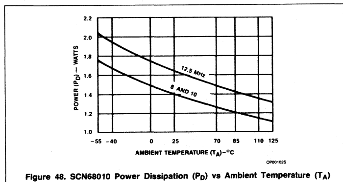
Figure 48. SCN68010 Power Dissipation (P D ) vs Ambient Temperature (T A )
