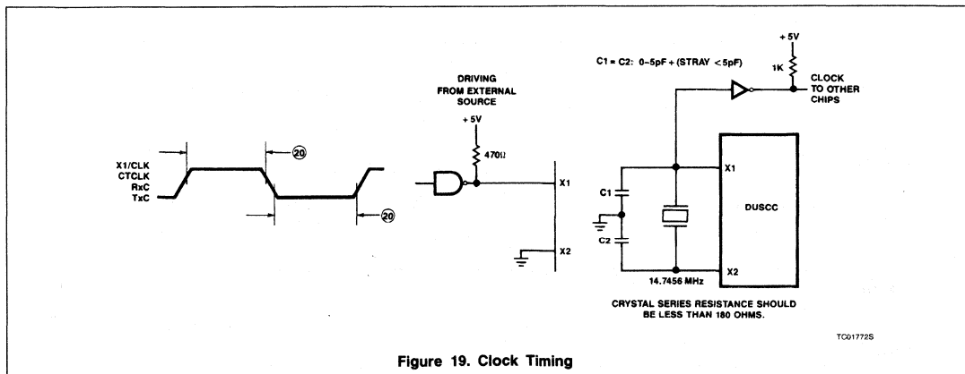
Figure 19. Clock Timing
