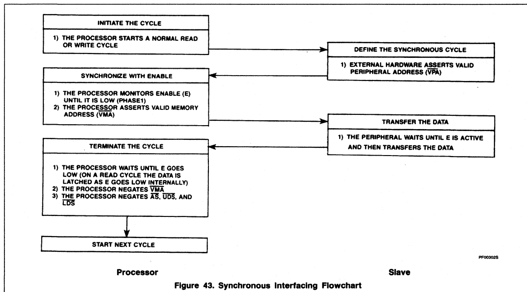
Figure 43. Synchronous Interfacing Flowchart
