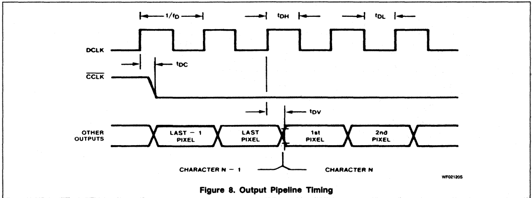
Figure 8. Output Pipeline Timing
