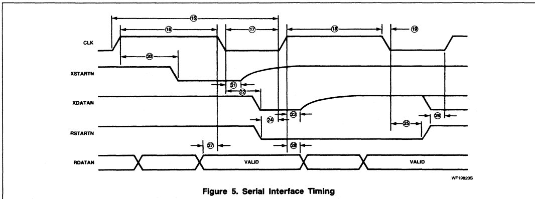
Figure 5. Serial Interface Timing
