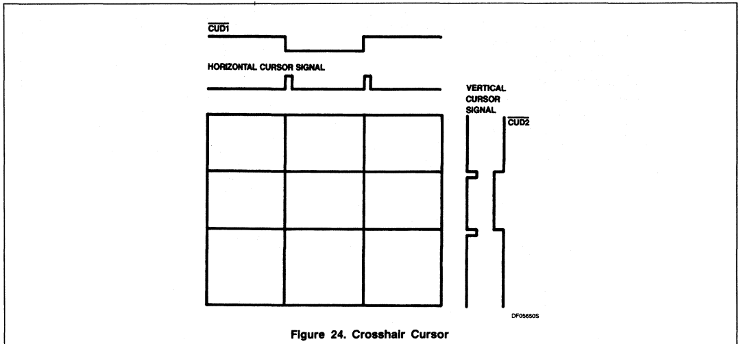
Figure 24. Crosshair Cursor
