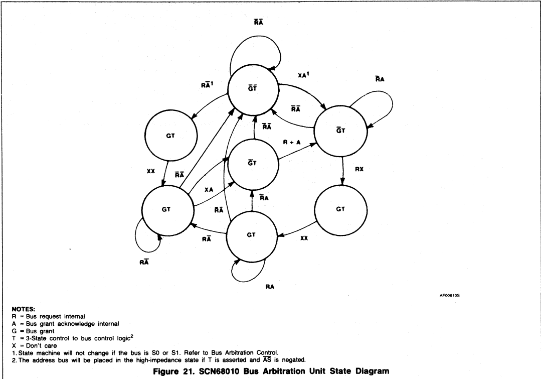
Figure 21. SCN68010 Bus Arbitration Unit State Diagram
