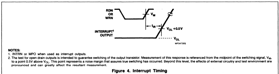
Figure 4. Interrupt Timing
