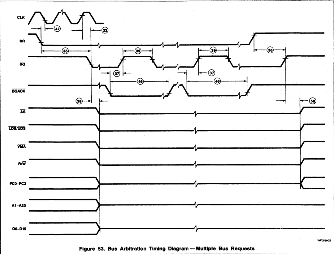
Figure 53. Bus Arbitration Timing Diagram — Multiple Bus Requests
