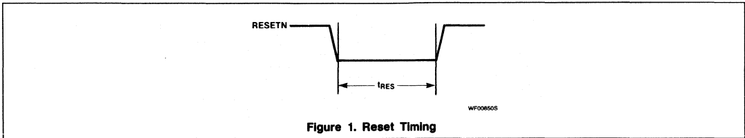
Figure 1. Reset Timing
