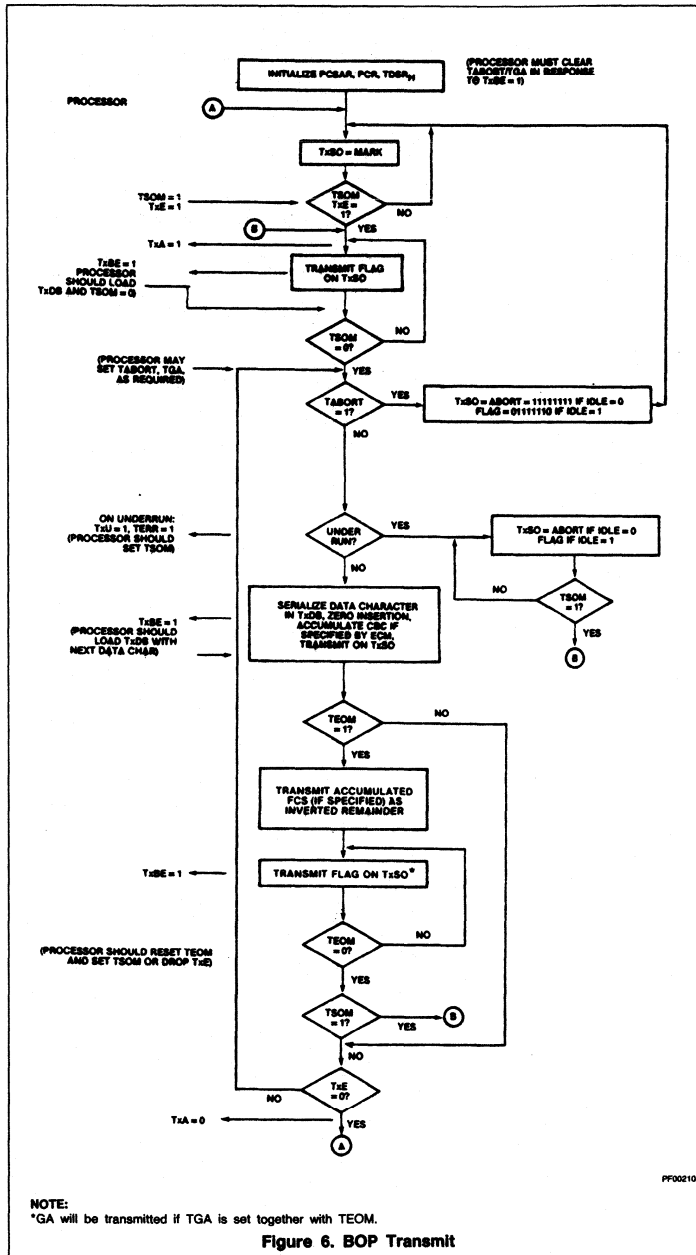
Figure 6. BOP Transmit
