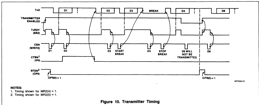
Figure 10. Transmitter Timing
