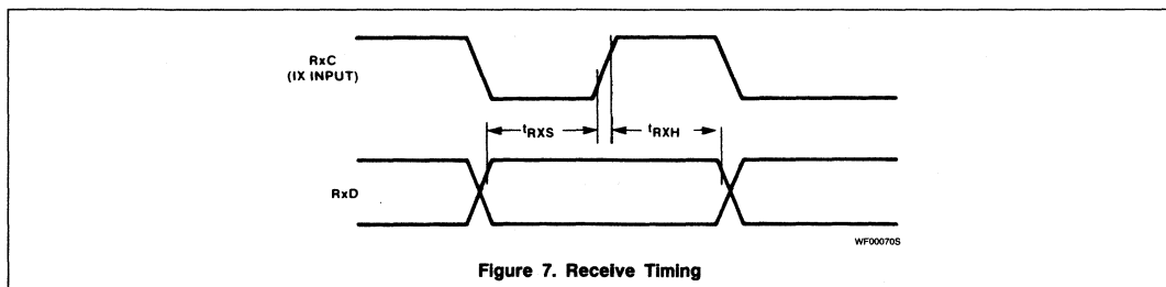
Figure 7. Receive Timing
