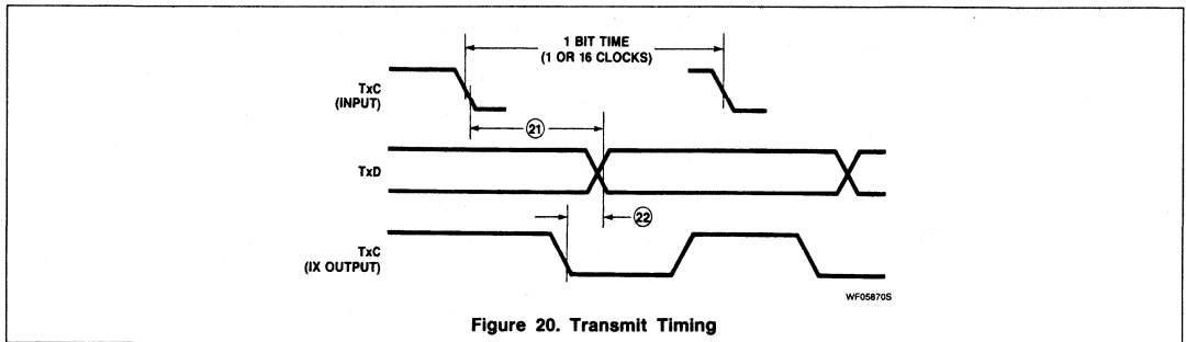
Figure 20. Transmit Timing
