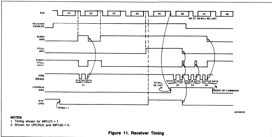
Figure 11. Receiver Timing
