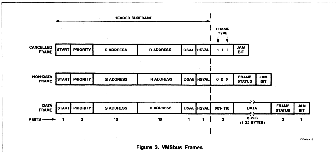
Figure 3. VMSbus Frames
