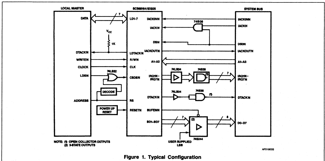
Figure 1. Typical Configuration
