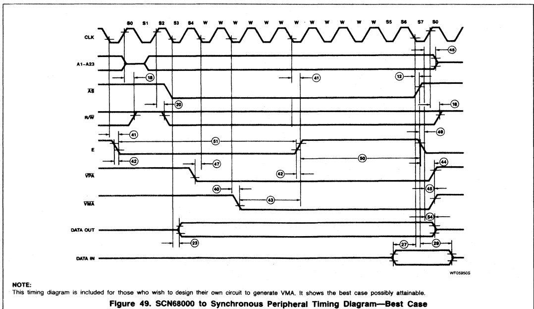
Figure 49. SCN68000 to Synchronous Peripheral Timing Diagram—Best Case
