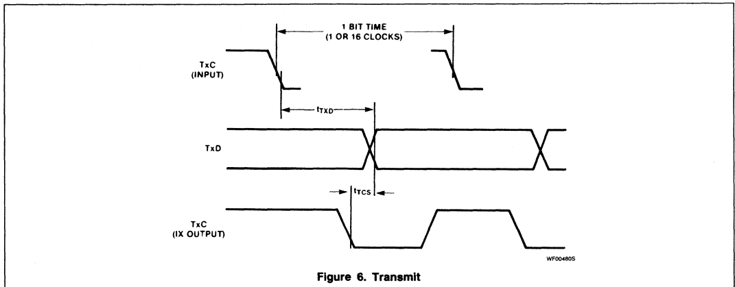
Figure 6. Transmit
