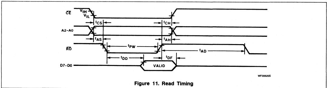
Figure 11. Read Timing
