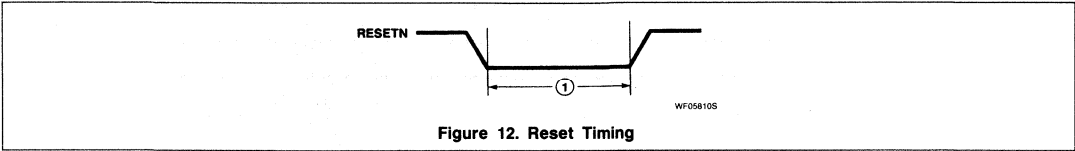
Figure 12. Reset Timing
