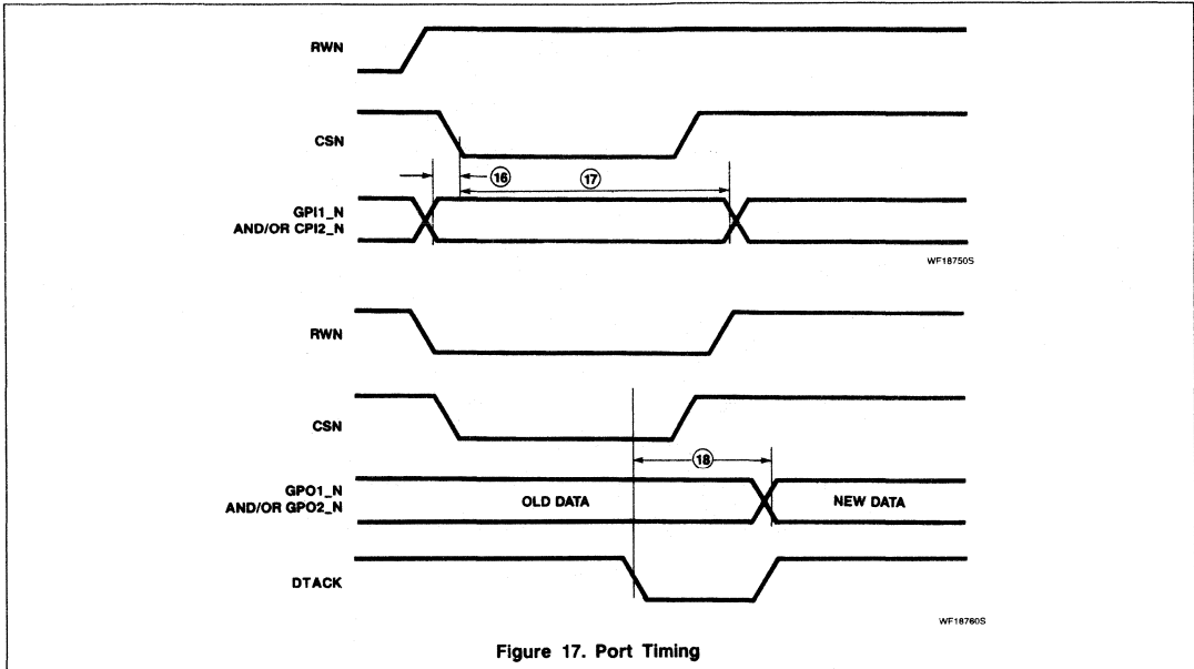
Figure 17. Port Timing
