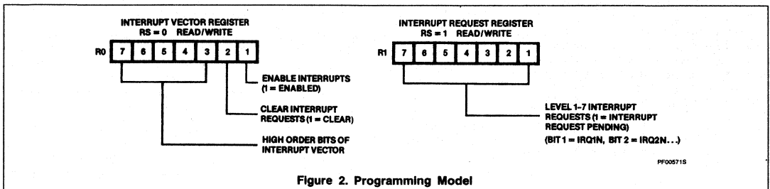
Figure 2. Programming Model
