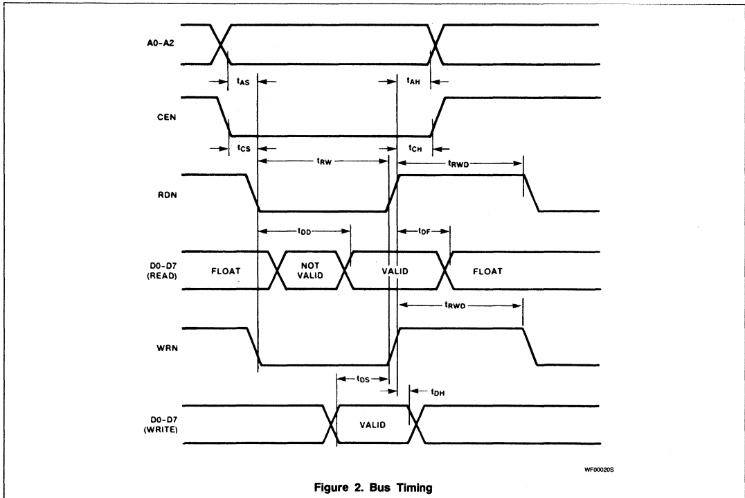
Figure 2. Bus Timing
