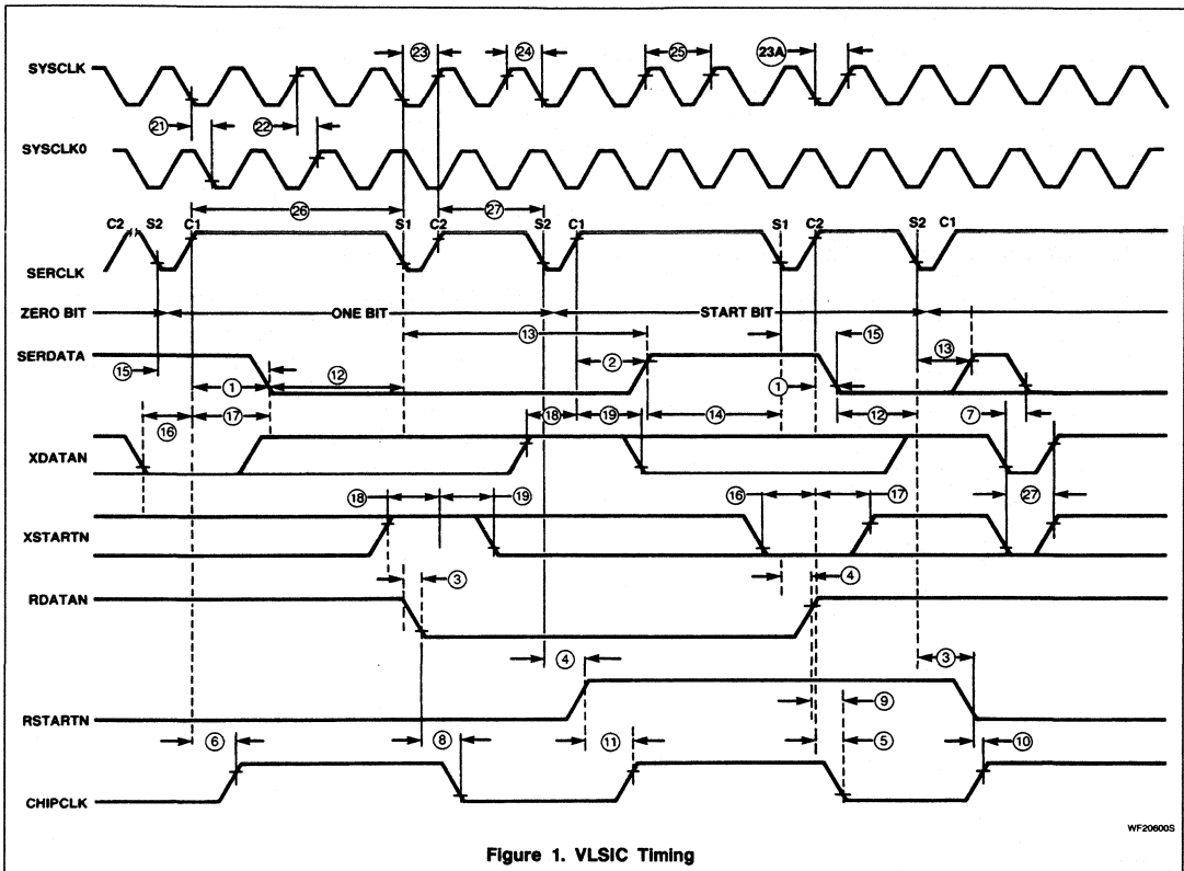
Figure 1. VLSIC Timing
