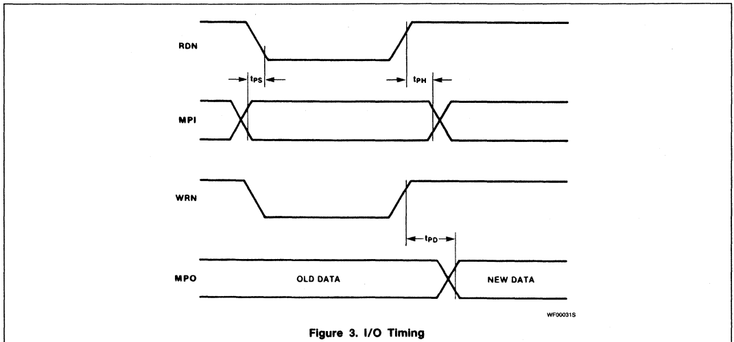
Figure 3. I/O Timing
