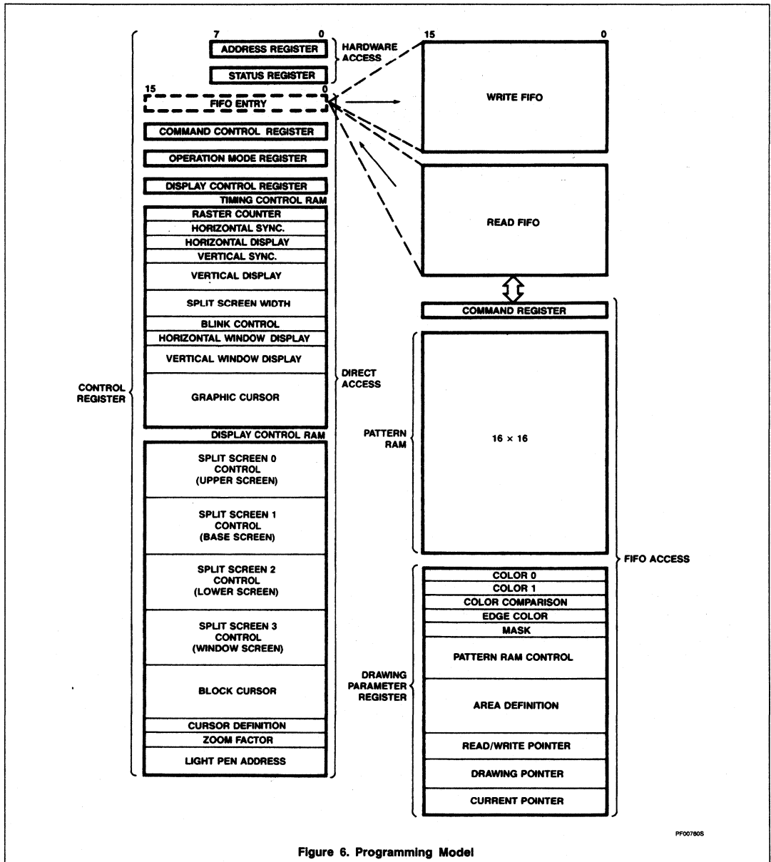
Figure 6. Programming Model
