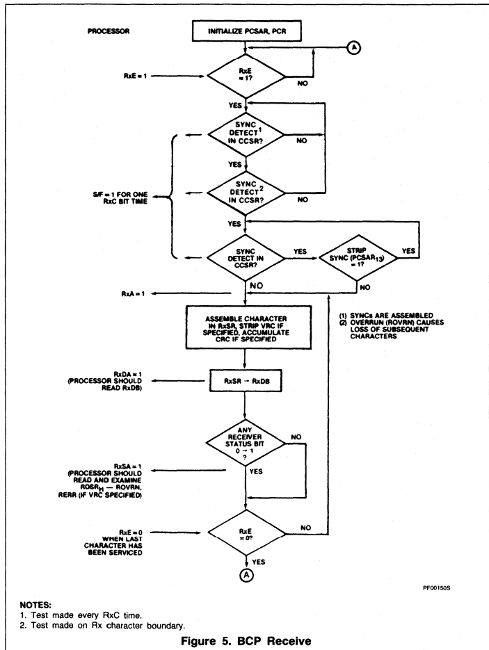
Figure 5. BCP Receive
