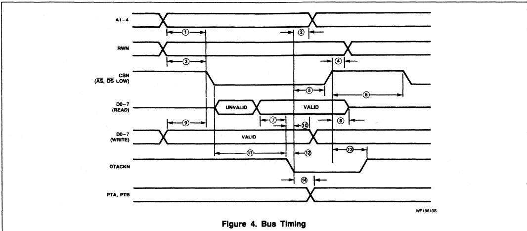
Figure 4. Bus Timing
