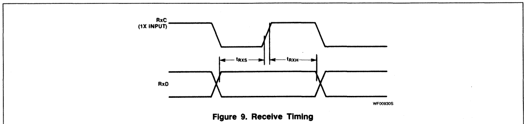
Figure 9. Receive Timing
