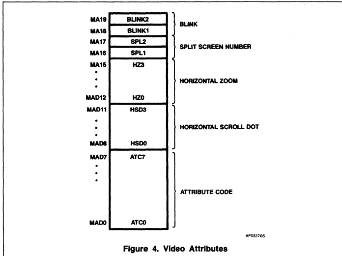
Figure 4. Video Attributes
