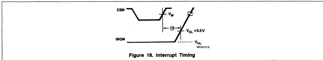
Figure 18. Interrupt Timing
