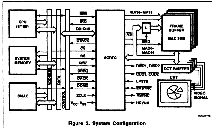
Figure 3. System Configuration
