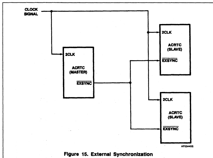
Figure 15. External Synchronization
