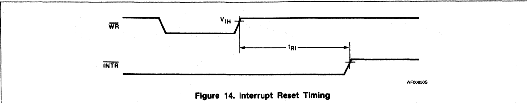
Figure 14. Interrupt Reset Timing
