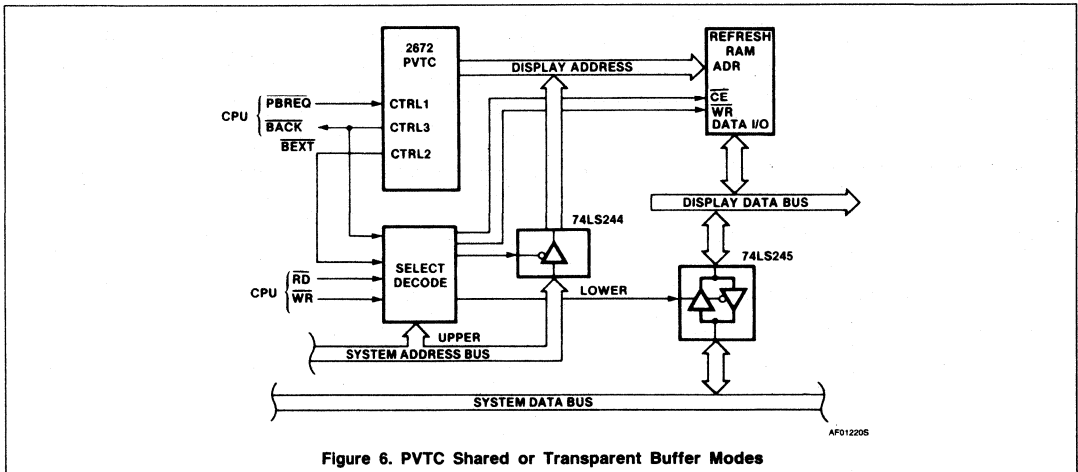
Figure 6. PVTC Shared or Transparent Buffer Modes
