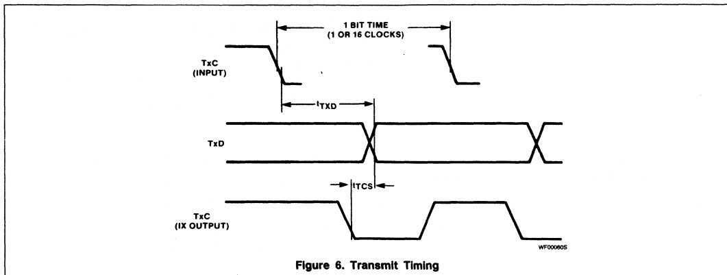
Figure 6. Transmit Timing
