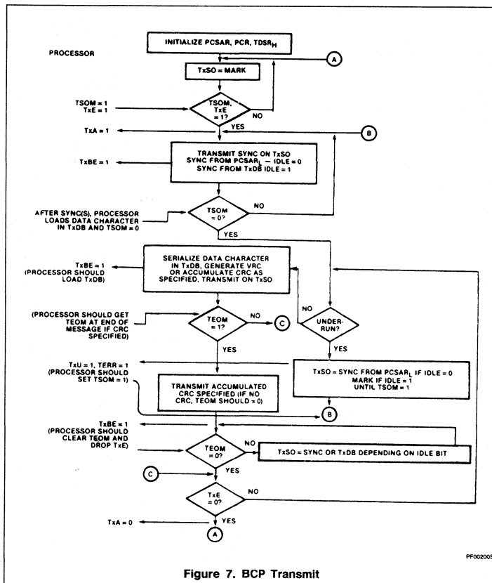
Figure 7. BCP Transmit
