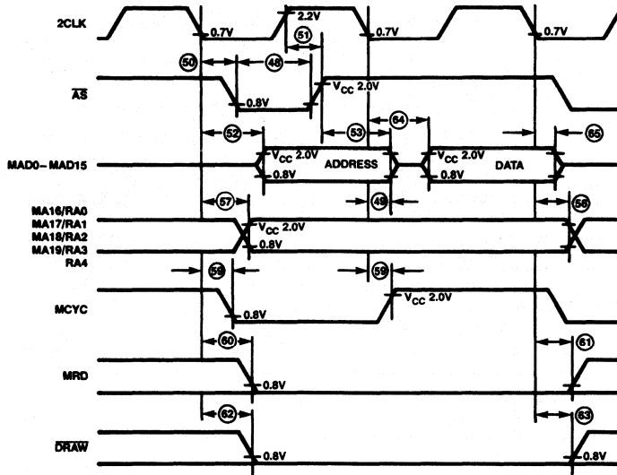
Figure 48. Frame Memory Write Cycle Timing (ACRTC → Frame Memory)
