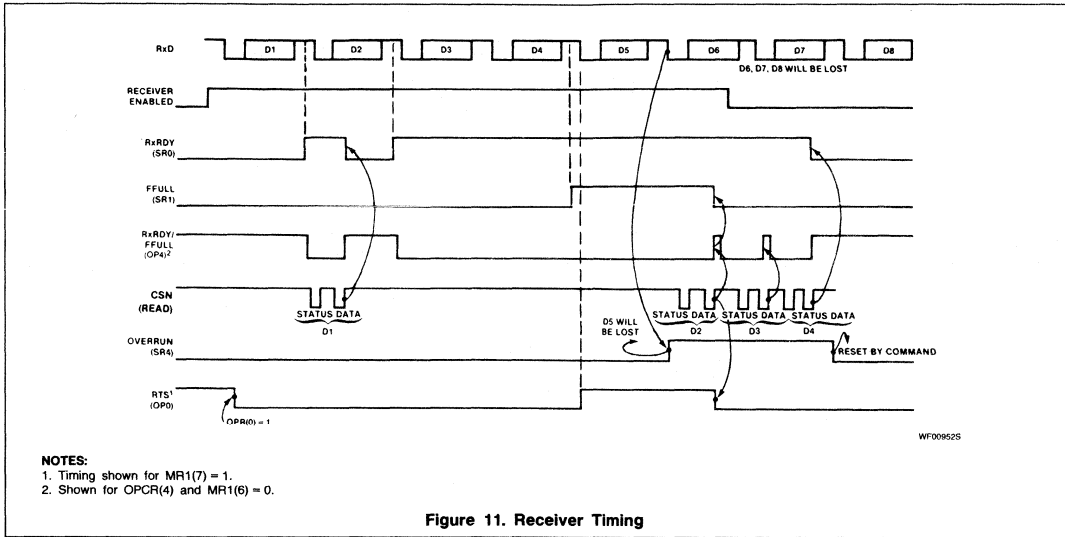
Figure 11. Receiver Timing
