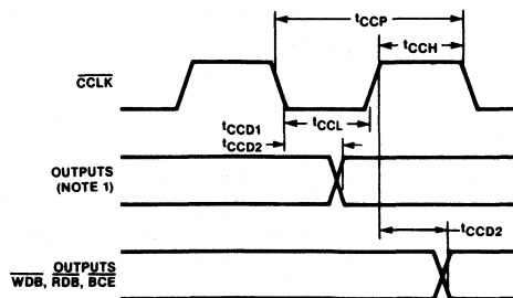
Figure 18. Bus Timing
