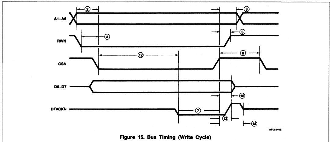
Figure 15. Bus Timing (Write Cycle)
