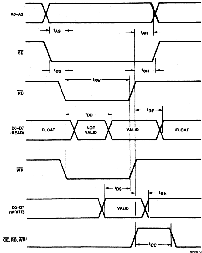
Figure 18. Bus Timing
