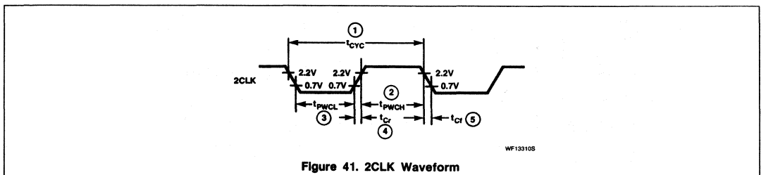
Figure 41. 2CLK Waveform
