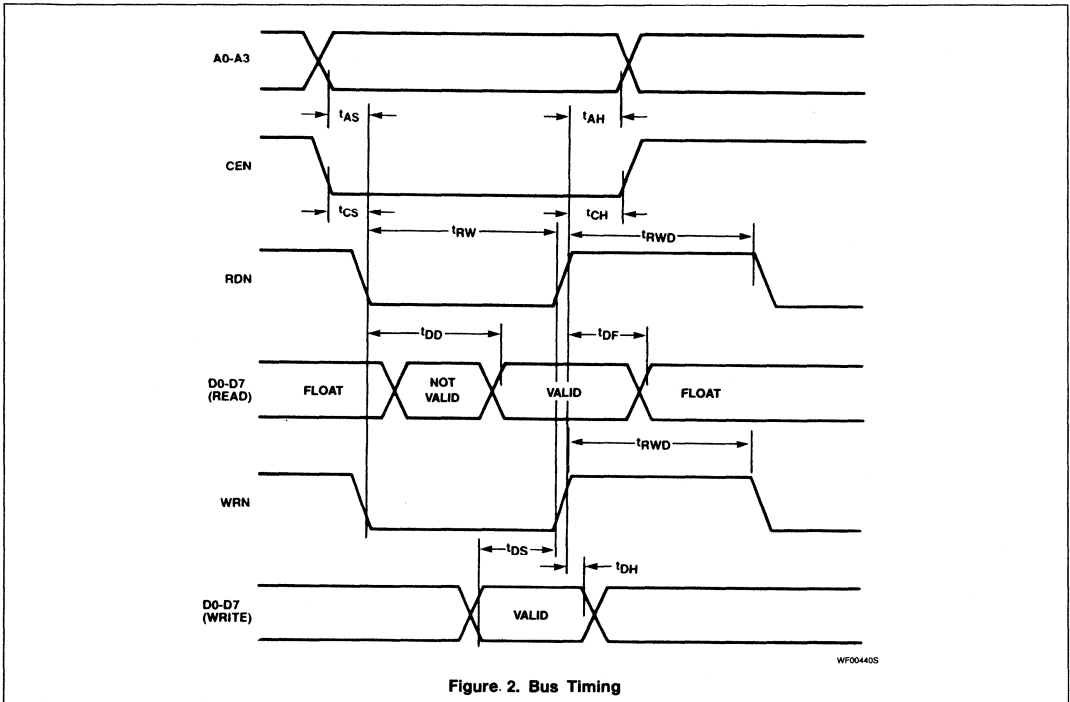
Figure 2. Bus Timing
