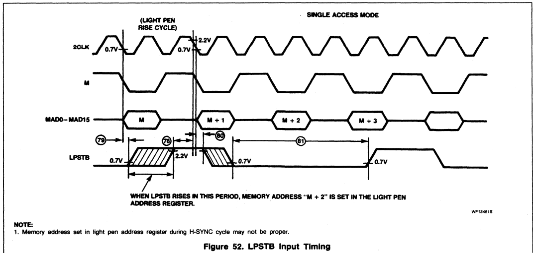
Figure 52. LPSTB Input Timing
