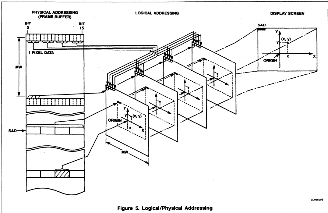
Figure 5. Logical/Physical Addressing
