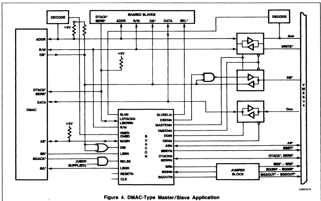
Figure 4. DMAC-Type Master/Slave Application
