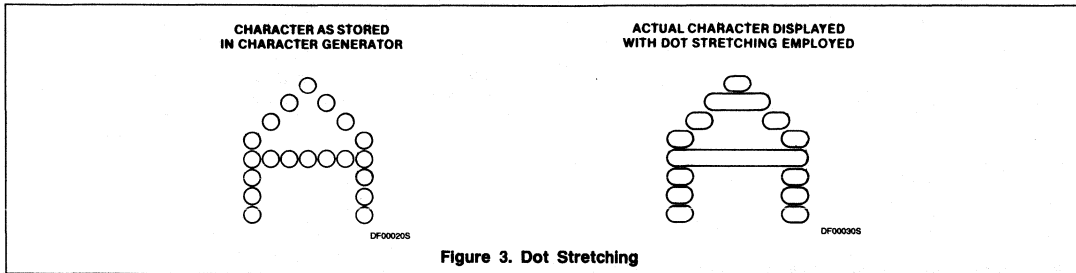
Figure 3. Dot Stretching
