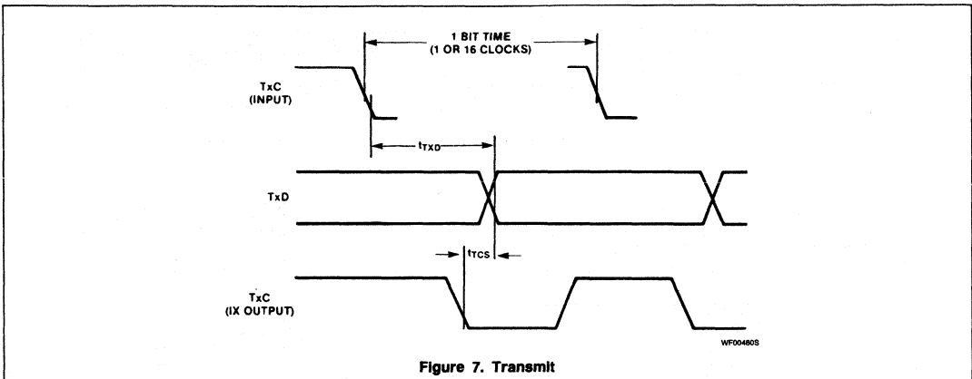
Figure 7. Transmit
