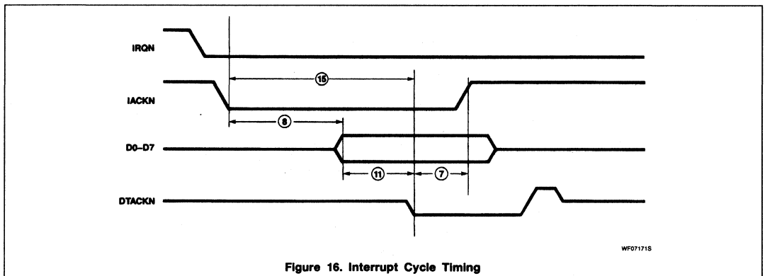
Figure 16. Interrupt Cycle Timing
