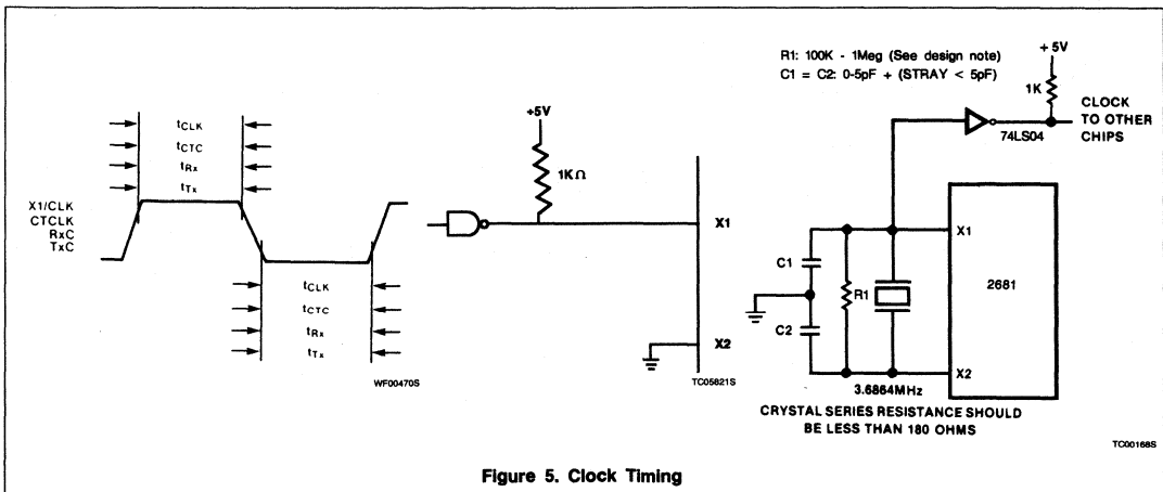
Figure 5. Clock Timing
