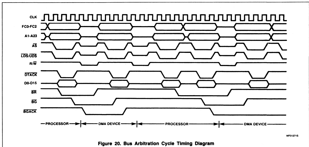
Figure 20. Bus Arbitration Cycle Timing Diagram
