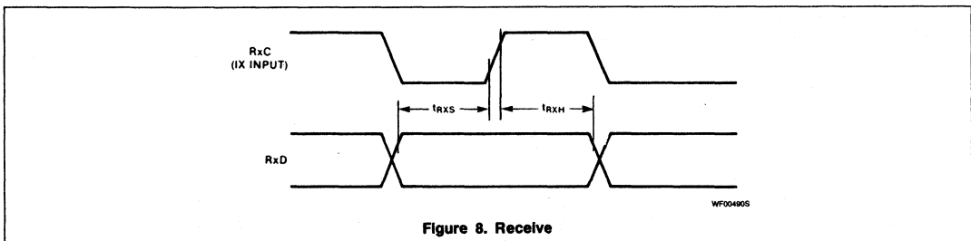
Figure 8. Receive
