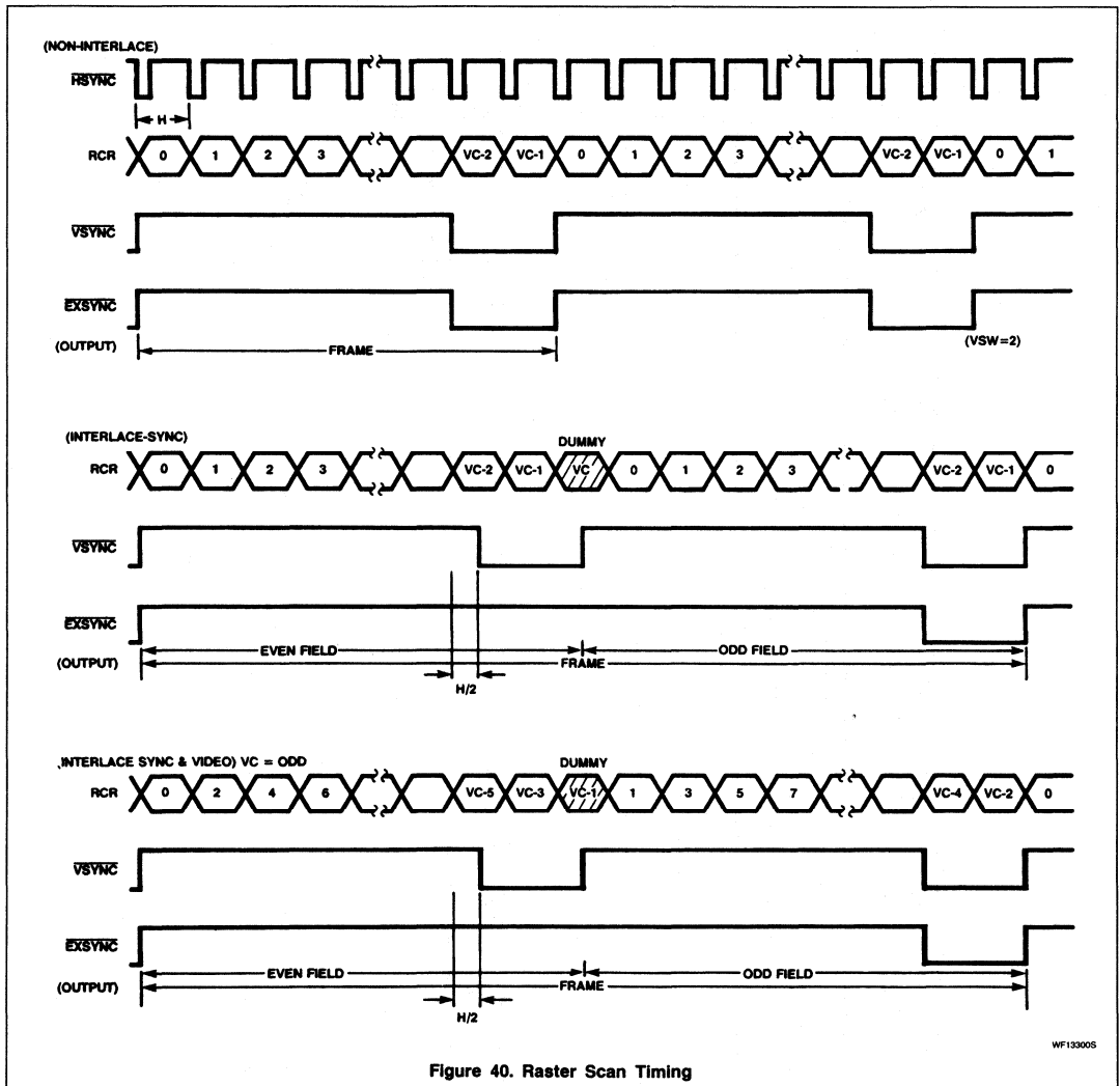
Figure 40. Raster Scan Timing
