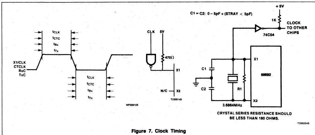
Figure 7. Clock Timing
