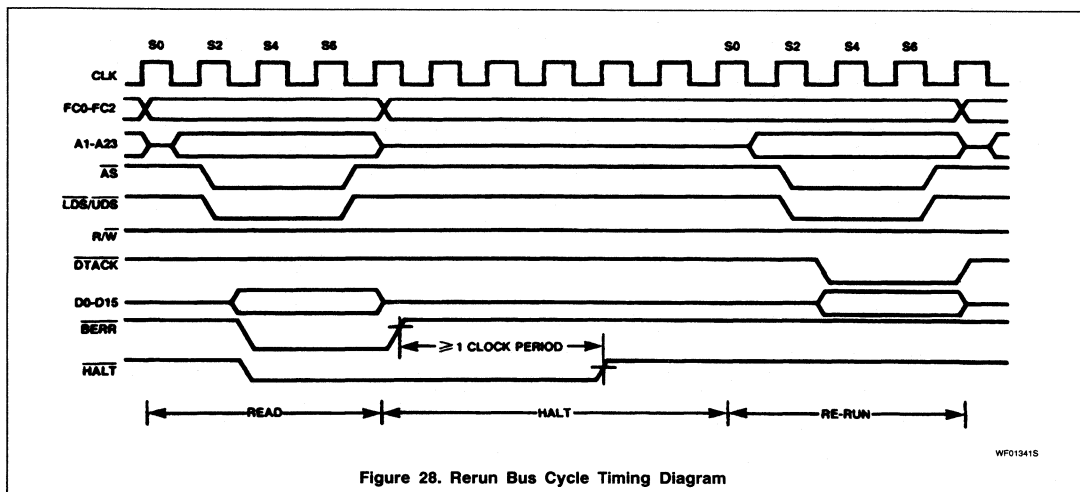
Figure 28. Rerun Bus Cycle Timing Diagram
