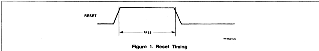
Figure 1. Reset Timing
