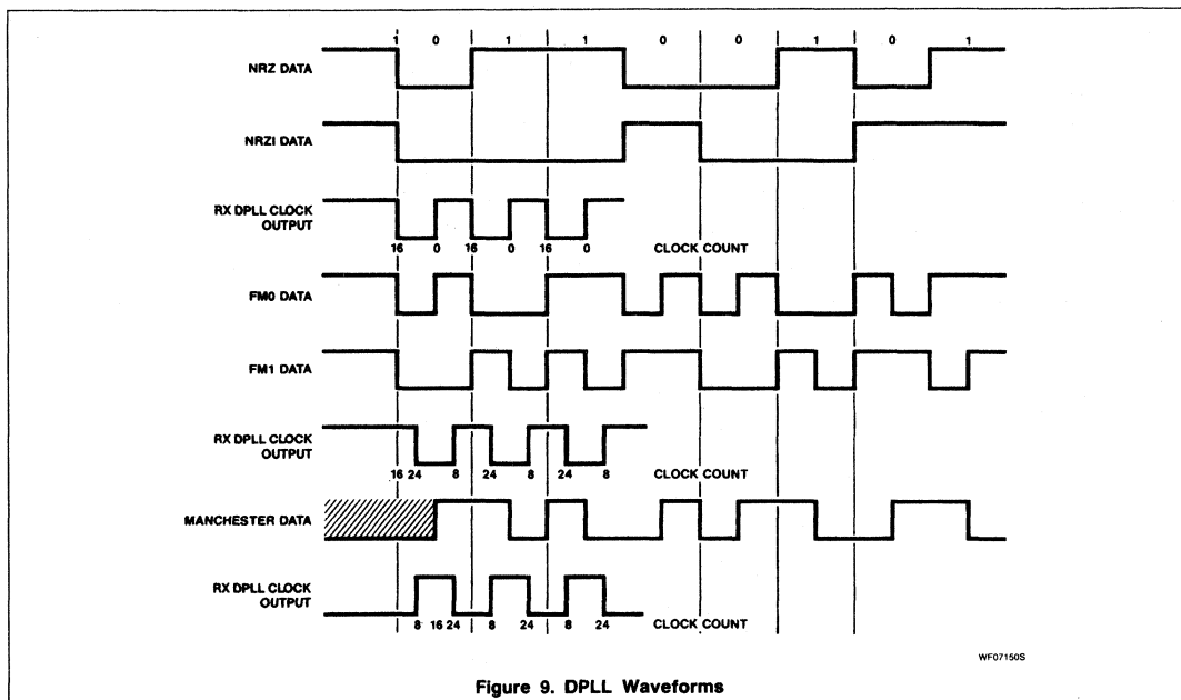
Figure 9. DPLL Waveforms
