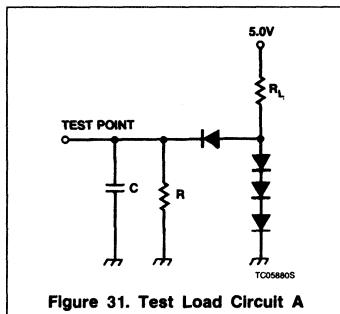
Figure 31. Test Load Circuit A
