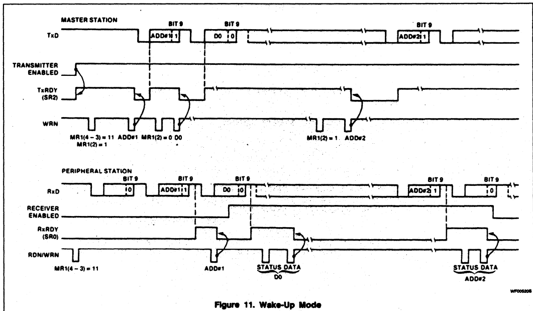
Figure 11. Wake-Up Mode
