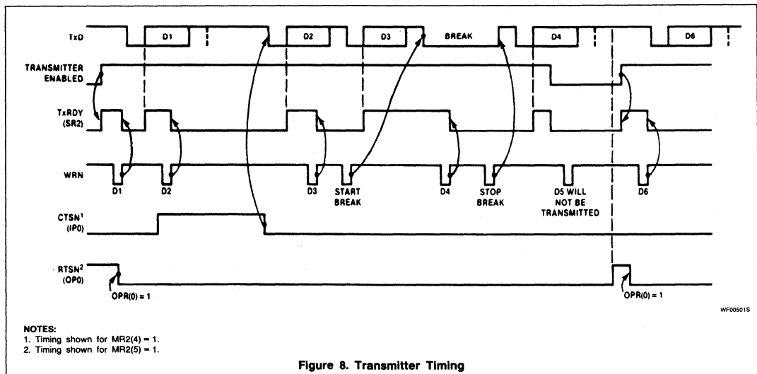
Figure 8. Transmitter Timing
