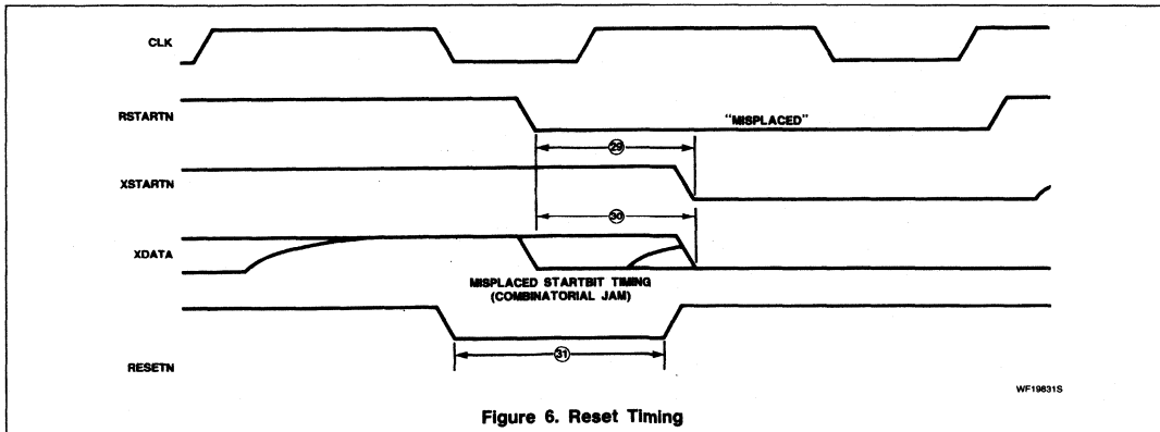
Figure 6. Reset Timing
