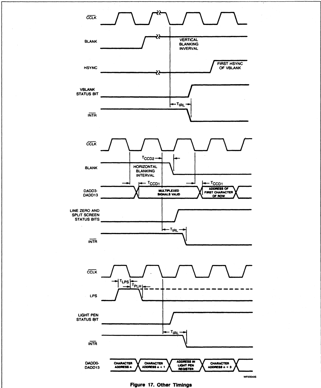
Figure 17. Other Timings
