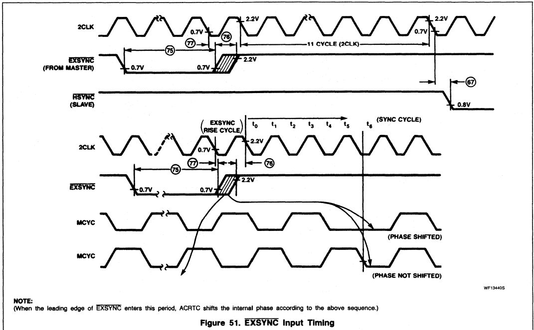
Figure 51. EXSYNC Input Timing
