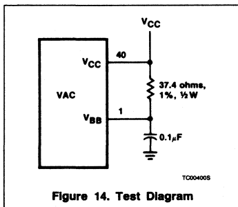
Figure 14. Test Diagram
