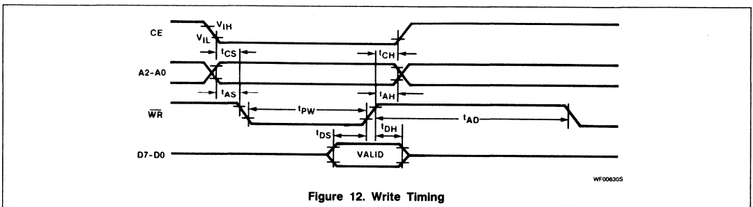
Figure 12. Write Timing
