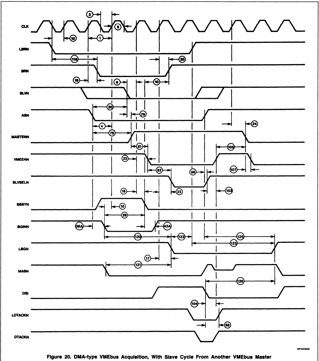
Figure 20. DMA-type VMEbus Acquisition, With Slave Cycle From Another VMEbus Master
