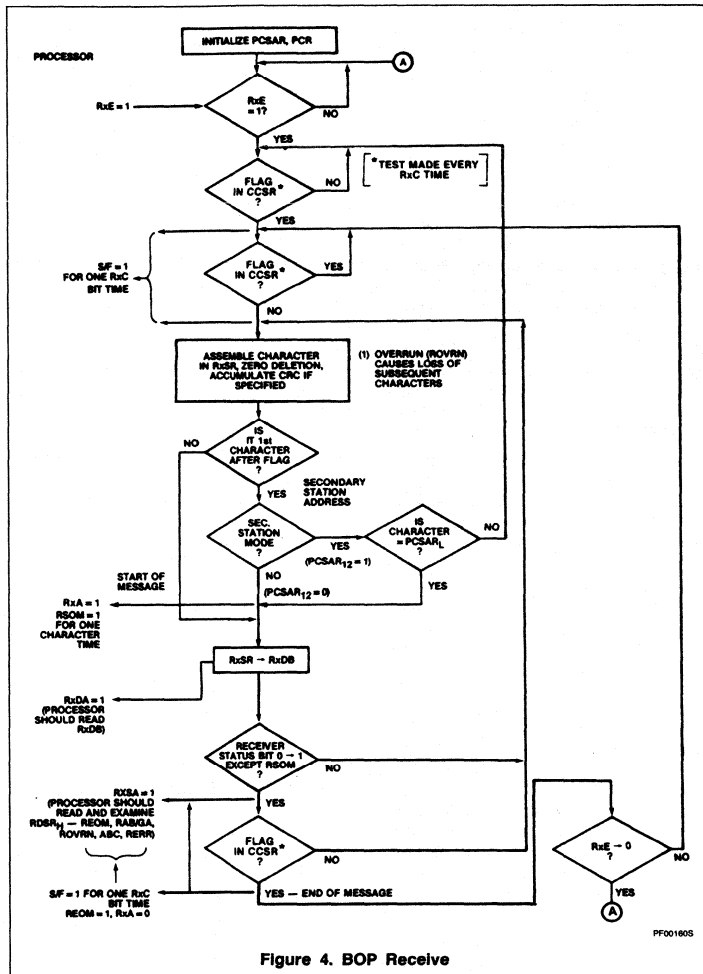
Figure 4. BOP Receive
