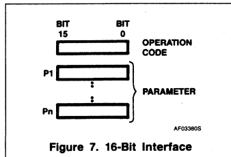
Figure 7. 16-Bit Interface
