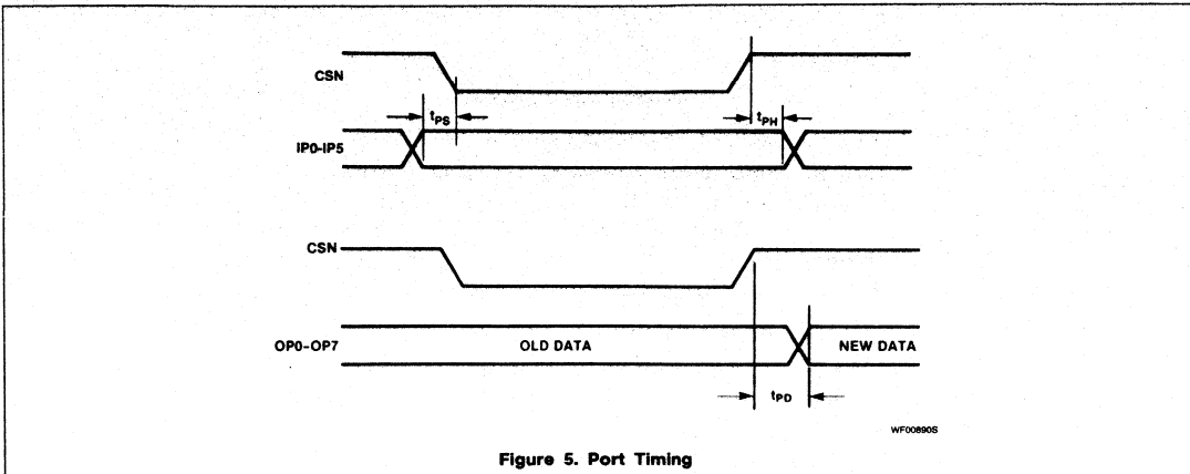
Figure 5. Port Timing
