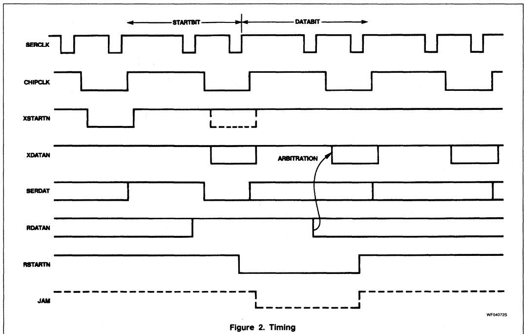
Figure 2. Timing
