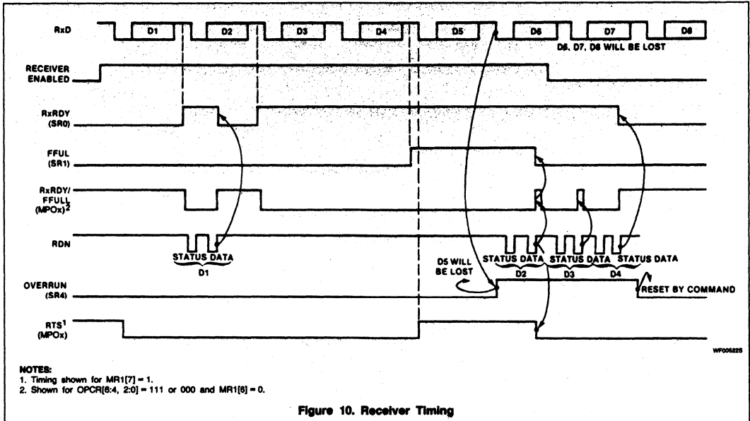
Figure 10. Receiver Timing
