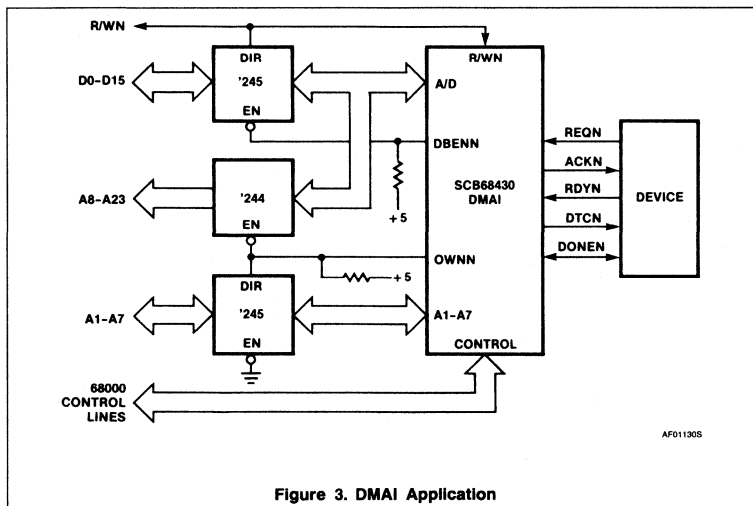
Figure 3. DMAI Application
